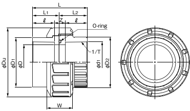
TS Socket-Thread (PVC)
