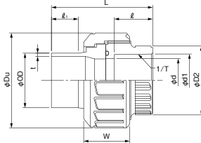
TS Socket-Butt(PVC-PVDF,HT-PVDF) PVDF Transition
